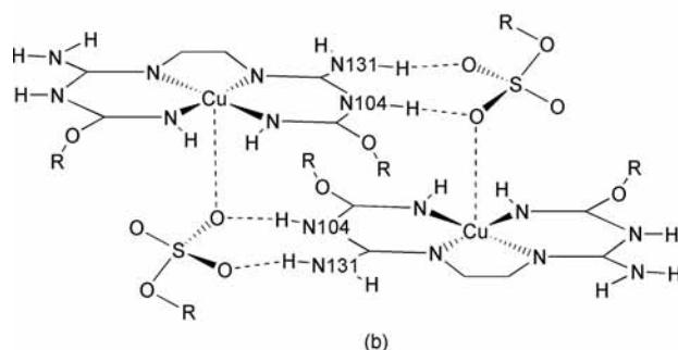
Scheme 4 Co-ordinative and hydrogen-bonding interactions linking copper(II) centres and hence sheets in compound 7 through (a) the co-ordinated imino nitrogens (N106, N206) and (b) the amino/imino (N131/N104) pair.
