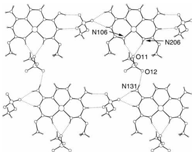
Fig. 3 Sheet structure of [\text{CuL}^{3m}][\text{MeOSO}_3]_2 7 .
