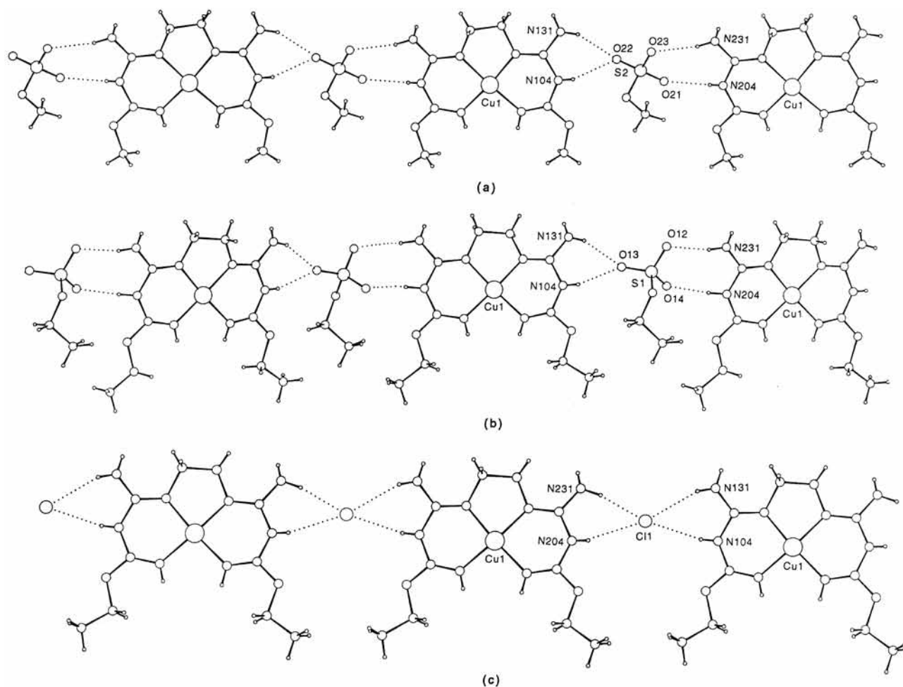
Fig. 2 Structures of the chains in (a) [\text{CuL}^{3m}][\text{MeOSO}_3]_2 7 , (b) [\text{CuL}^{3e}][\text{EtOSO}_3]_2 8 and (c) [\text{CuL}^{3e}][\text{EtOSO}_3]\text{Cl}\cdot 2\text{H}_2\text{O} 9 showing the hydrogen bonded supramolecular synthons.
