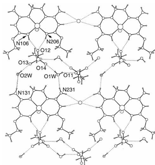
Fig. 4 Sheet structure of [\text{CuL}^{3e}][\text{EtOSO}_3]\text{Cl}\cdot 2\text{H}_2\text{O} 9 .
