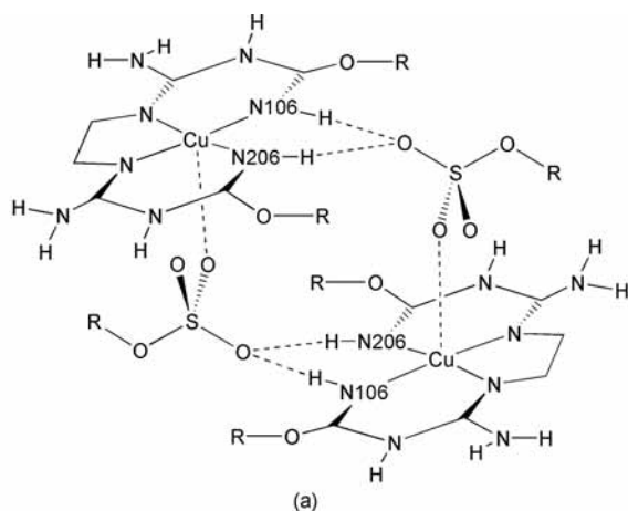
Fig. 5 Parallel packing of the sheets in [\text{CuL}^{3m}][\text{MeOSO}_3]_2 7 showing the co-ordinative and hydrogen-bonding interactions involved in the generation of the framework structure.
