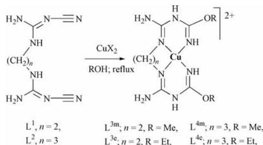
Scheme 1 Synthesis of [\text{CuL}^i]^{2+} cations.
